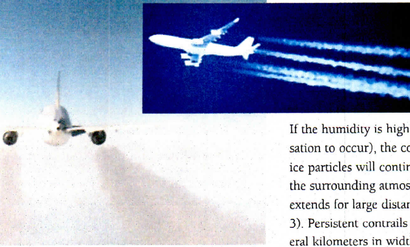
Figure 1. Contrails forming behind the engines of a Lufthansa Airbus A310-330 cruising at an altitude of 35,100 ft (10.7 km) as seen from research aircraft. (Photo: German Aerospace Center (Deutsches Zentrum für Luft- und Raumfahrt (DLR)), Oberpfaffenhofen, Germany.) Inset: Contrails forming behind the engines of a large commercial aircraft. Typically, contrails become visible within roughly a wingspan distance behind the aircraft. (Photo: Masako Imai, Cloud Castle/Photo Sky Japan.)
